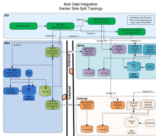
Figure 8–2 Sender Side Split Topology
