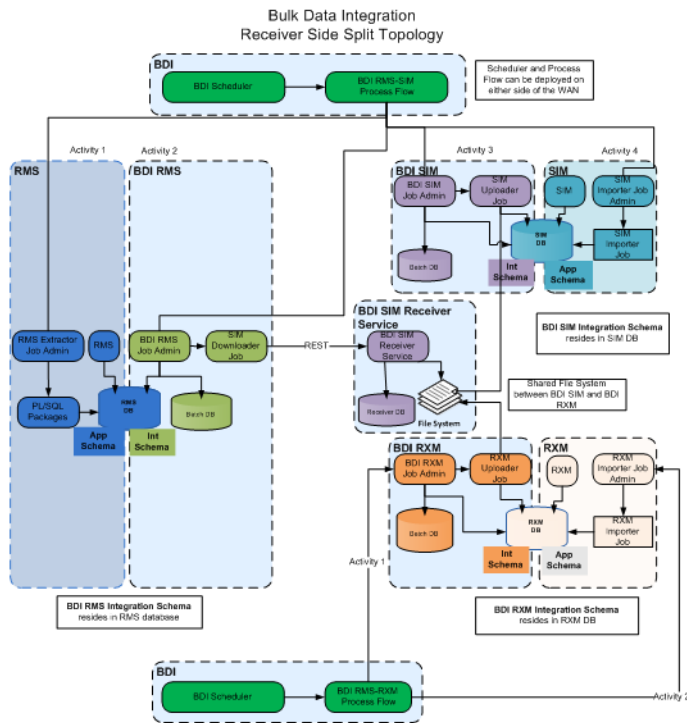
Figure 8-4 Receiver Side Split
